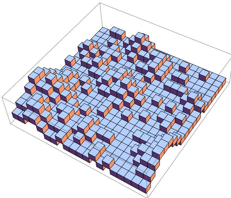
Fig. 1. Part of the lowest open Lipschitz surface (on a finite torus) when d = 3 and p = 0.82 . Each cube represents an open site in the surface.
