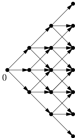
Fig. 2. Part of the lattice \vec{\mathbb{L}}_{\text{alt}}^2 of [13], obtained by adding oriented edges to \mathbb{Z}^2 .
