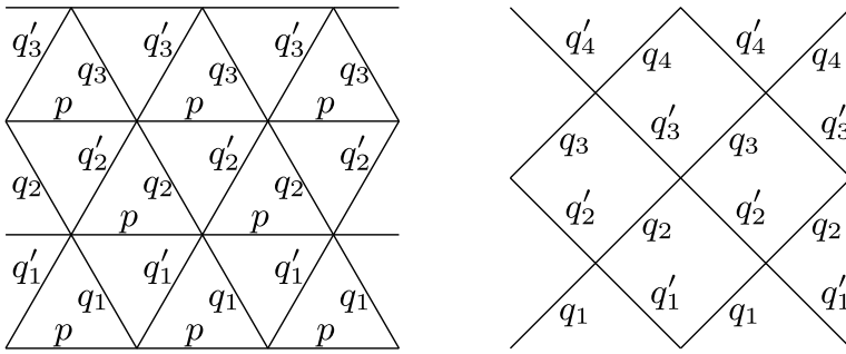
FIG. 2. Left: The triangular lattice with the highly inhomogeneous product measure \mathbb{P}_{p, \mathbf{q}, \mathbf{q}'} . The probability for each edge to be open is described in the picture: all horizontal edges have probability p of being open, while the other edges have probability q_n (right edges of upward pointing triangles) or q'_n (left edges of upward pointing triangles) of being open, with n being their height. Right: The square lattice with a highly inhomogeneous product measure \mathbb{P}_{\mathbf{q}, \mathbf{q}'} , rotated by \pi/4 . Edges inclined at angle \pi/4 have probability q_n of being open, while edges inclined at angle 3\pi/4 have probability q'_n of being open, with n being their height.
