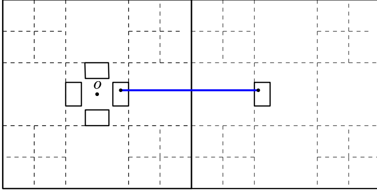
FIGURE 5.6. The regions T_{e_i} , 6re_1 + T_{-e_1} , and the event C_{e_1} .
