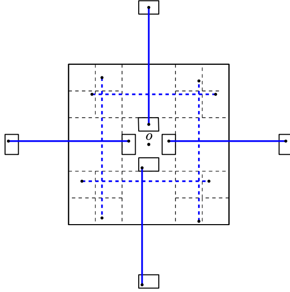
FIGURE 5.7. The event C(o) is depicted in solid lines, and A(o) in dashed lines.
