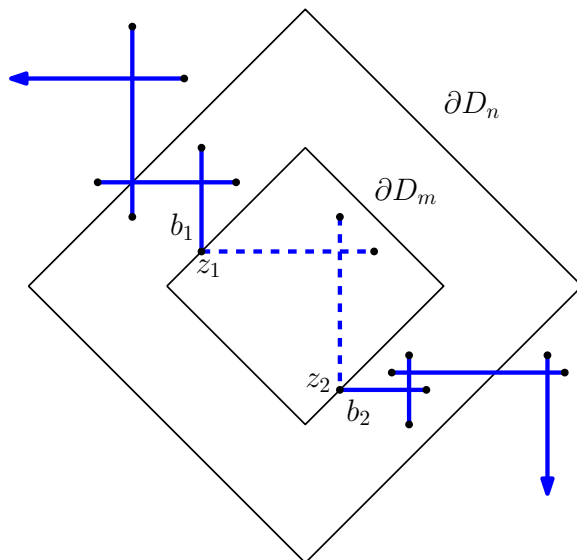
FIGURE 5.1. An illustration of the proof of statement B in Theorem 5.1. The dashed lines indicate the blue segments created within D_m to connect z_1 and z_2 . The arrows indicate connections to infinity.
