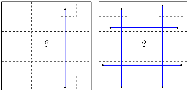
FIGURE 5.5. The events A_{e_1} and A(o) .
