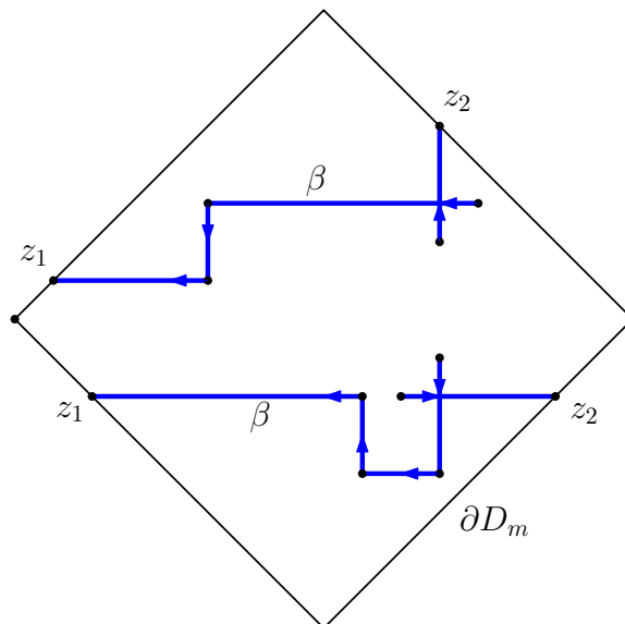
FIGURE 5.2. (i) The upper picture is an illustration of the creation of a blue path from z_1 to z_2 when the graph-geodesic \gamma has some number r \geq 1 of changes of direction. (ii) The lower picture illustrates the case r = 0 .
