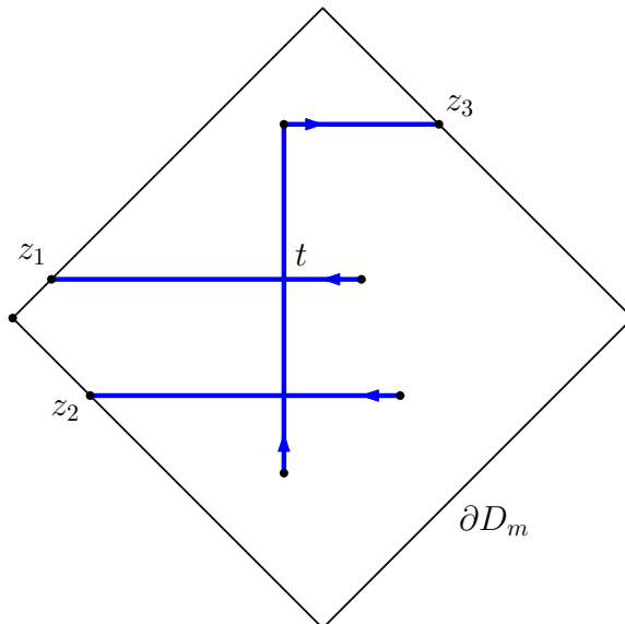
FIGURE 5.4. An illustration of the special construction when two of the z_i are close to one another.
