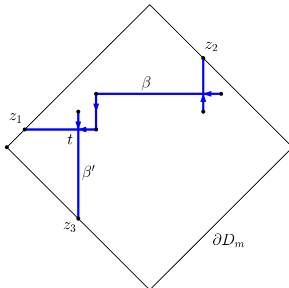
FIGURE 5.3. An illustration of the construction of a trifurcation in the proof of statement C. A geodesic from z_1 to z_2 is transformed into a sequence \beta of blue segments. Similarly, a geodesic from z_3 to \beta is transformed into a sequence \beta' of blue segments.
